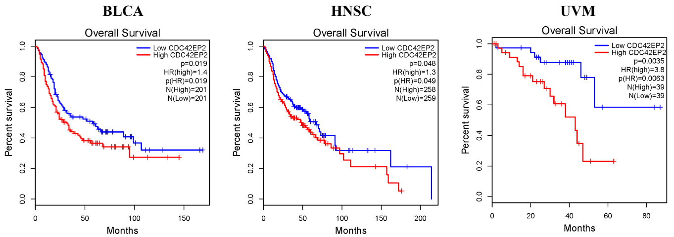
Figure S2. Prognostic value of CDC42 effector protein 2 (CDC42EP2) expression in several cancers. The prognostic significance of CDC42EP2 expression was analyzed using the GEPIA2 database. BLCA, bladder urothelial carcinoma; HNSC, head and neck squamous cell carcinoma; UVM, uveal melanoma; HR, hazard ratio.
